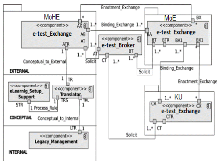
Fig. 3. E-Assessment architecture based on NREN [13].
