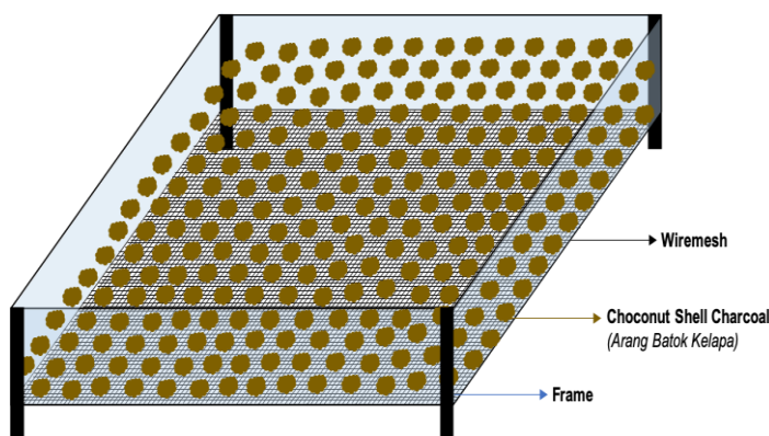
Figure 4. The final design of charcoal filter
